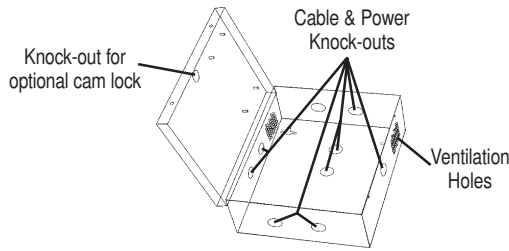
FIG. 1 — Enclosure Knock-outs
