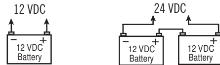
FIG. 2 — Back-up Battery Configuration.
