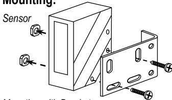
Mounting with Bracket
